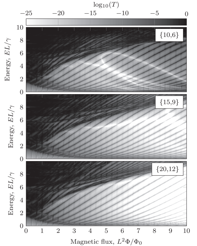
FIG. 7. Transmittance of \{10,6\} , \{15,9\} , and \{20,12\} triangular GABs in scaled units.
