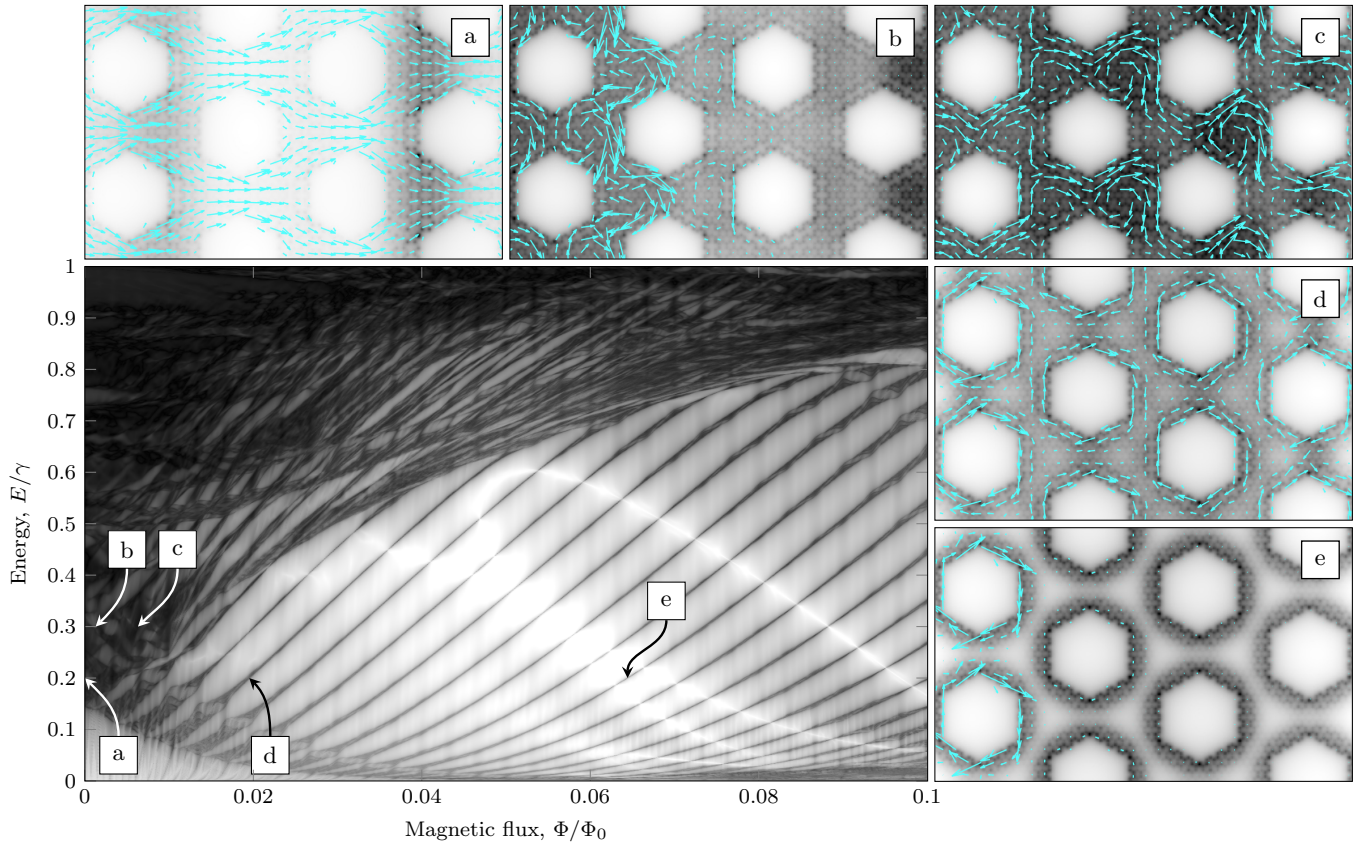
FIG. 5. LDOS (gray shading) and bond current (blue arrows) of a \{10,6\} triangular GAB for different B -field strengths at energies of (a),(d),(e) E = 0.2\gamma or (b),(c) E = 0.3\gamma . The main panel shows the transmittance of the system. Here, we plot \sqrt{|\log_{10}(T)|} in order to enhance the contrast.
